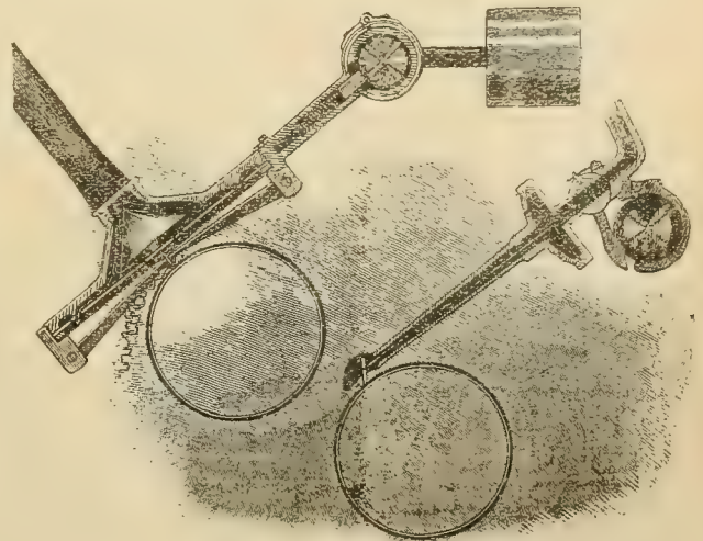
FIG. 2.—RECORDING AND REPRODUCING MECHANISM.
